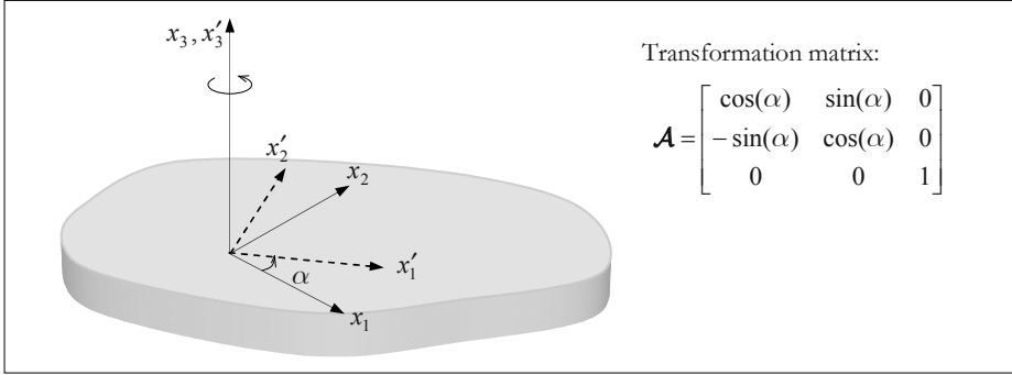
Figure 7.4: Transversely isotropic symmetry.
