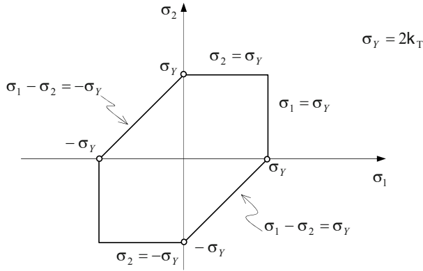
Figure 9.12: Tresca yield curve – Plane stress.
