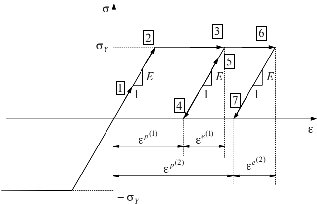
Figure 9.28: One-dimensional perfect plasticity.
