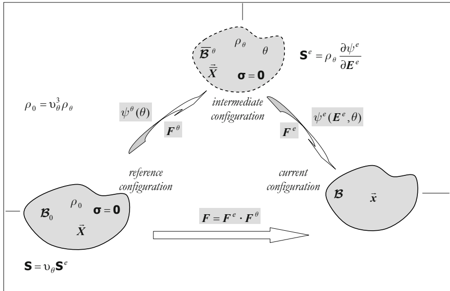
Figure 10.9: Energy, stress and mass density in different configurations.
