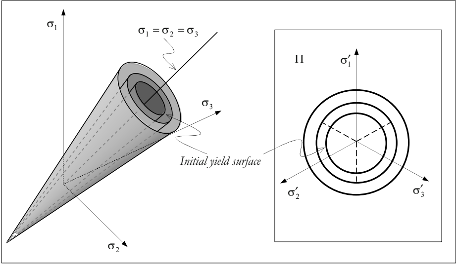
Figure 9.26: Evolution of the yield surface in the Drucker-Prager model with isotropic hardening.
