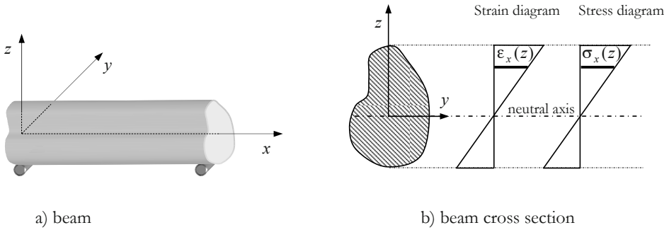
Figure 7.22: Beam.
