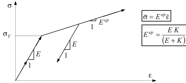
Figure 9.36: Elastoplastic tangent stiffness modulus.
