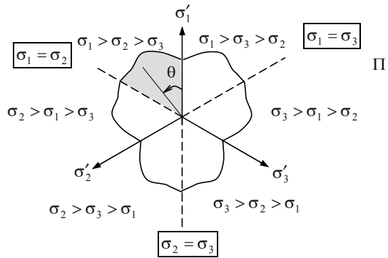
Figure 9.5: Yield surface projected onto a \Pi -plane.
