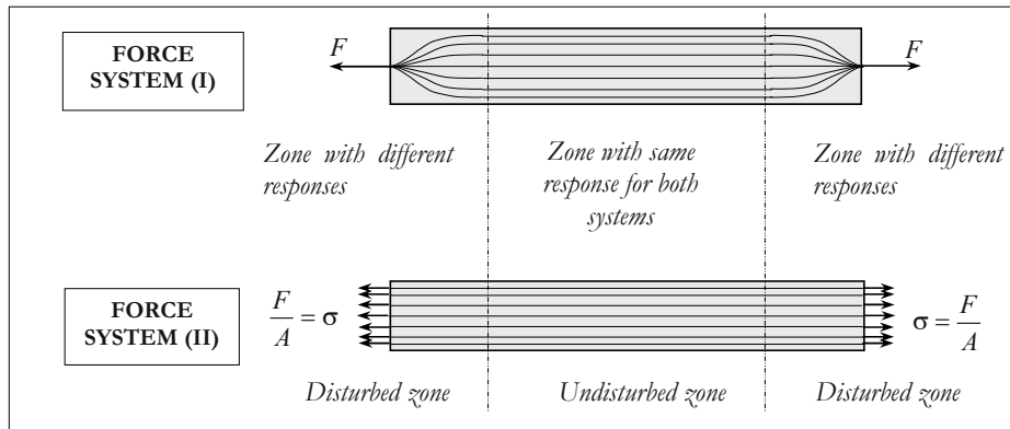
Figure 7.10: Saint-Venant's principle.
