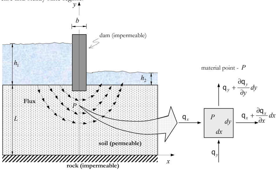
Figure 5.15: Fluid flow throughout the porous medium.
