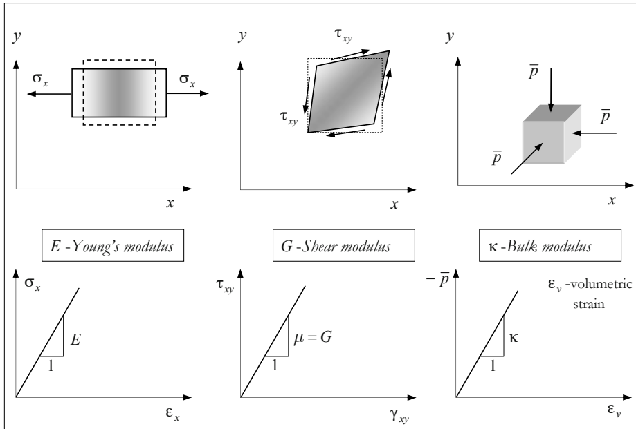
Figure 7.7: Some material mechanical properties.
