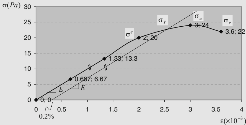
Figure 6.13: Stress-strain curve.
