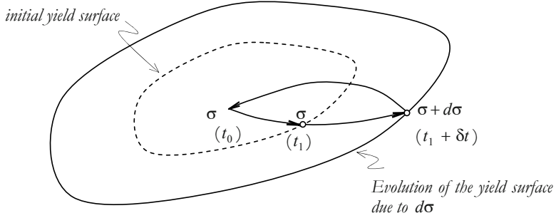
Figure 9.40: Evolution of the yield surface.
