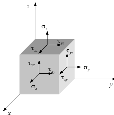
Figure 3.9: Stress state at a point P – Engineering notation.
