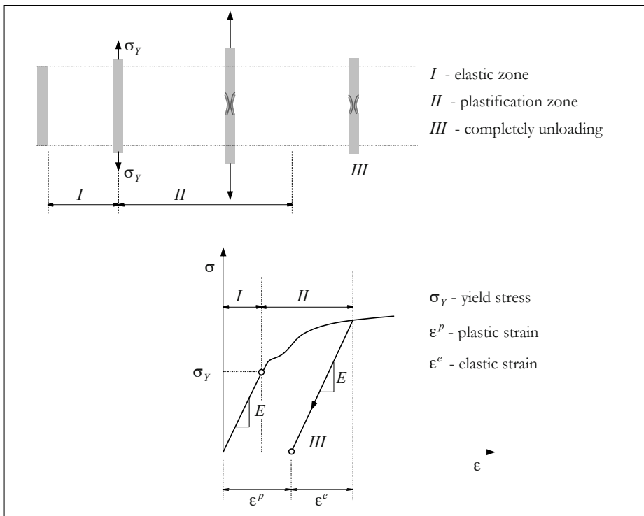
Figure 6.7: Elastoplastic behavior.
