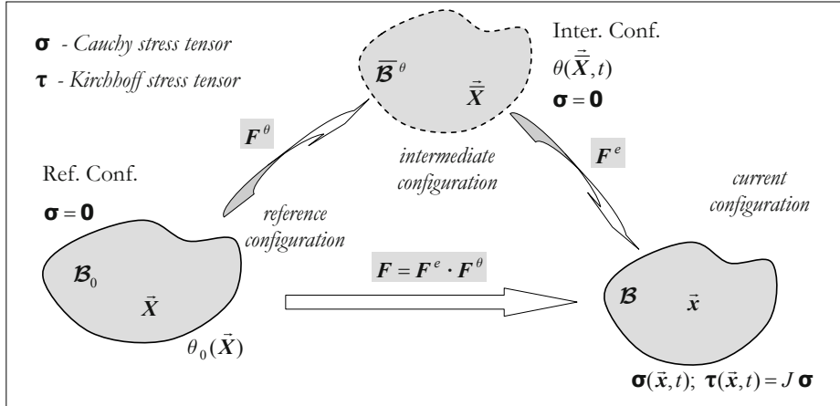
Figure 10.6: Multiplicative decomposition.
