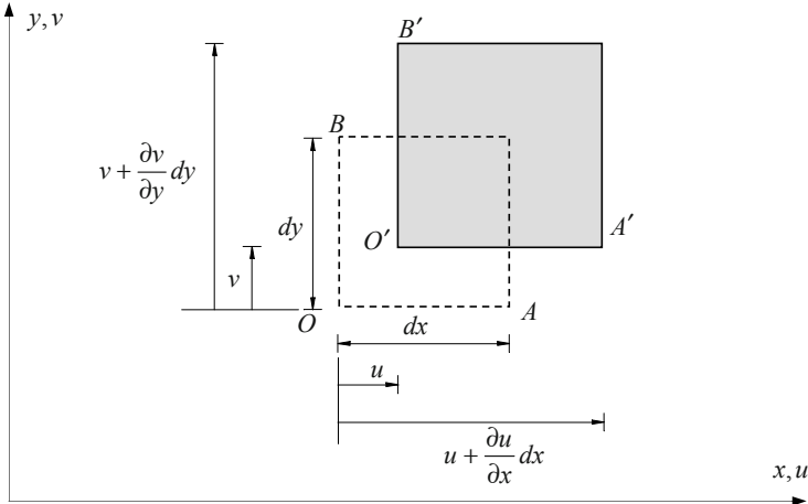
Figure 2.37: Normal strain.
