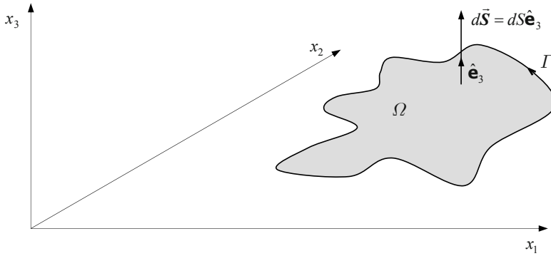
Figure 1.42: Green's theorem.
