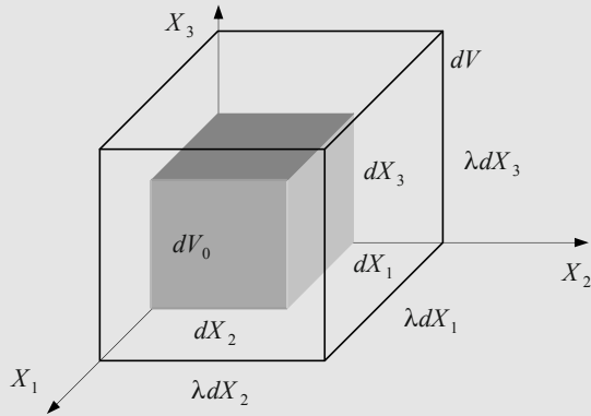
Figure 8.7: Dilatation.
