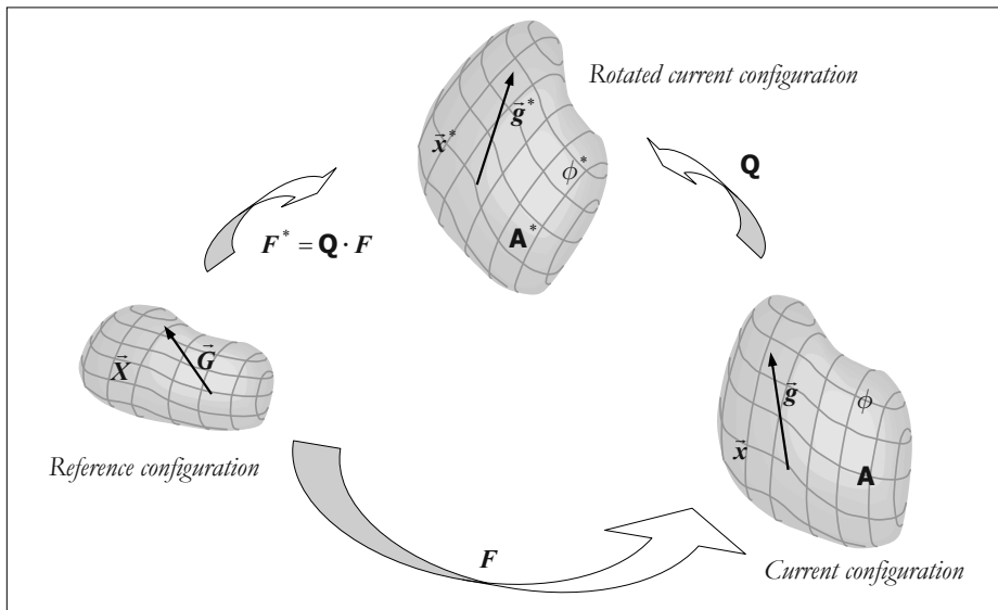
Figure 4.2: Motions.
