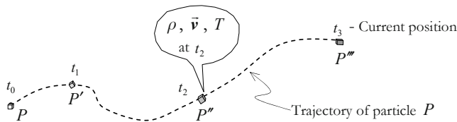
Figure 2.3: Particle trajectory.
