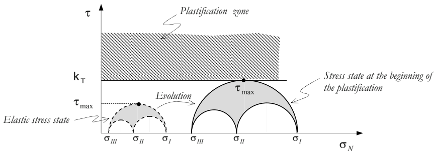
Figure 9.9: The Tresca yield criterion.
