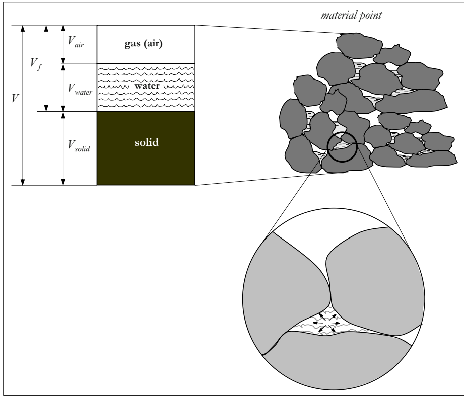
Figure 6.19: Porous material.
