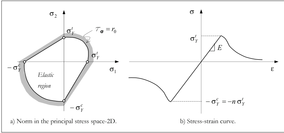
Figure 11.12: Damage surface in 2D and the uniaxial stress-strain curve for model III.
