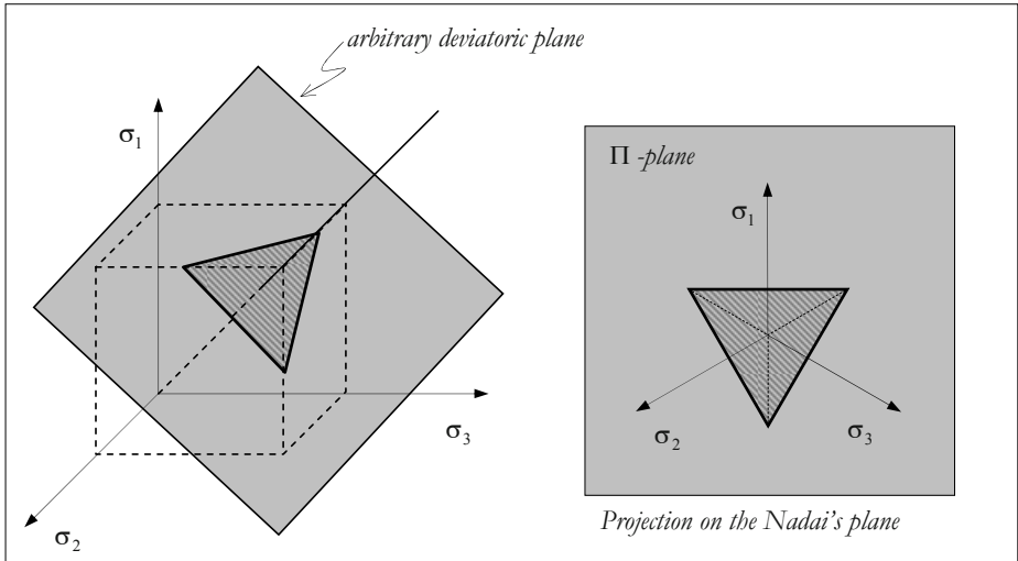
Figure 9.23: The Rankine yield criterion.
