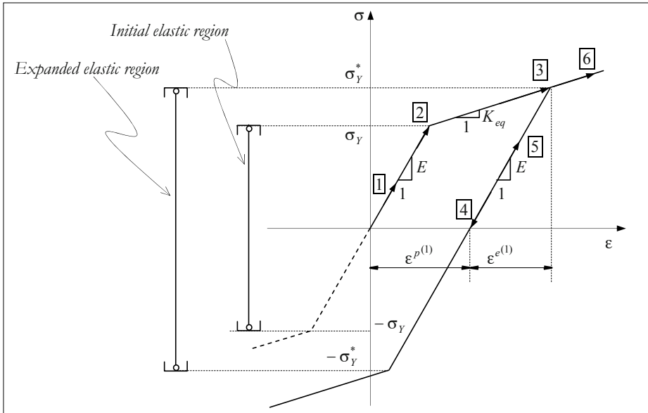
Figure 9.32: Isotropic hardening elastoplastic behavior.
