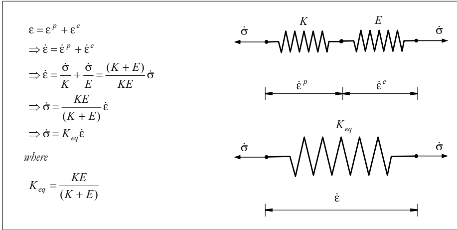
Figure 9.34: Linear springs disposed in series.
