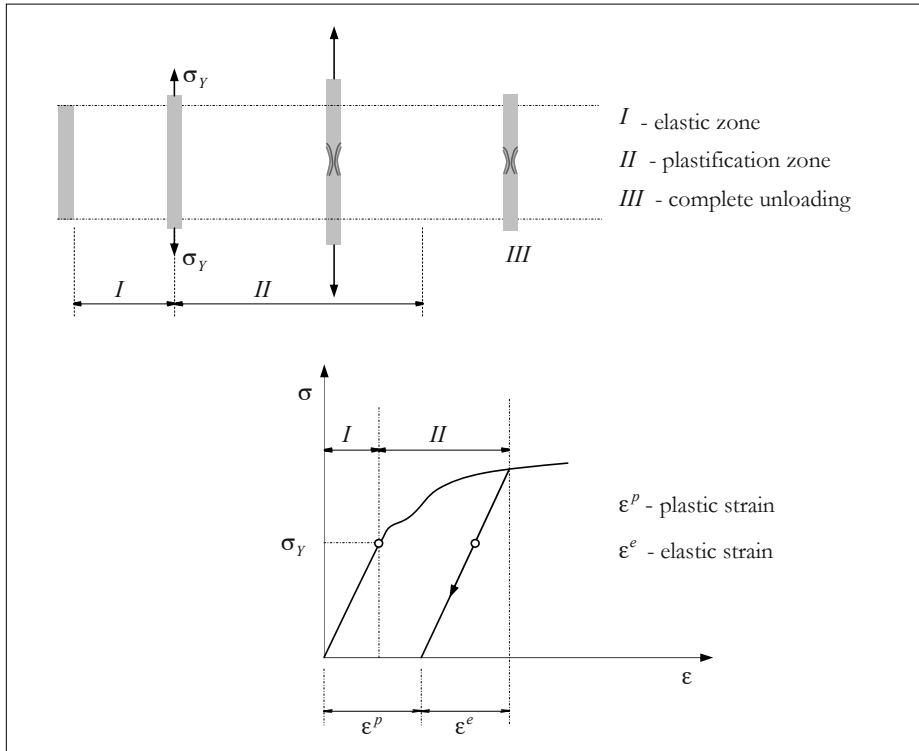
Figure 9.1: Tensile testing – Plastic behavior.
