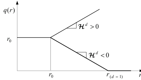
Figure 11.7: The linear hardening/softening law.
