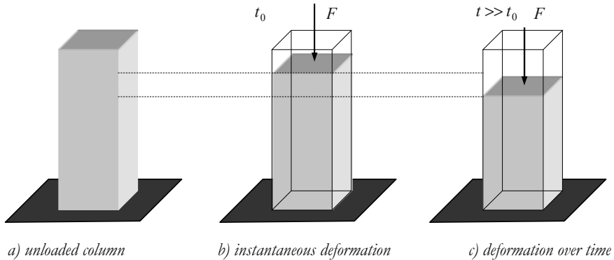
Figure 6.21: Creep phenomenon.
