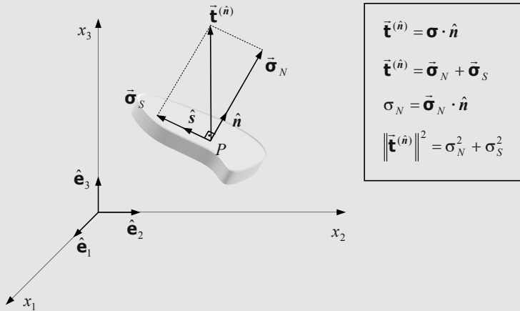
Figure 3.12: Normal and tangential stress vector.
