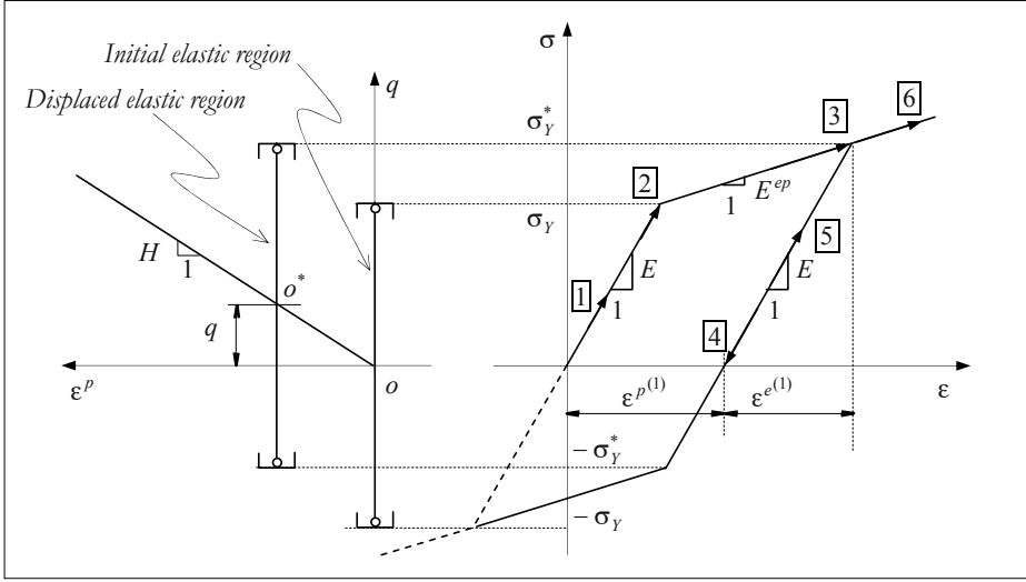
Figure 9.37: Kinematic hardening elastoplastic behavior.
