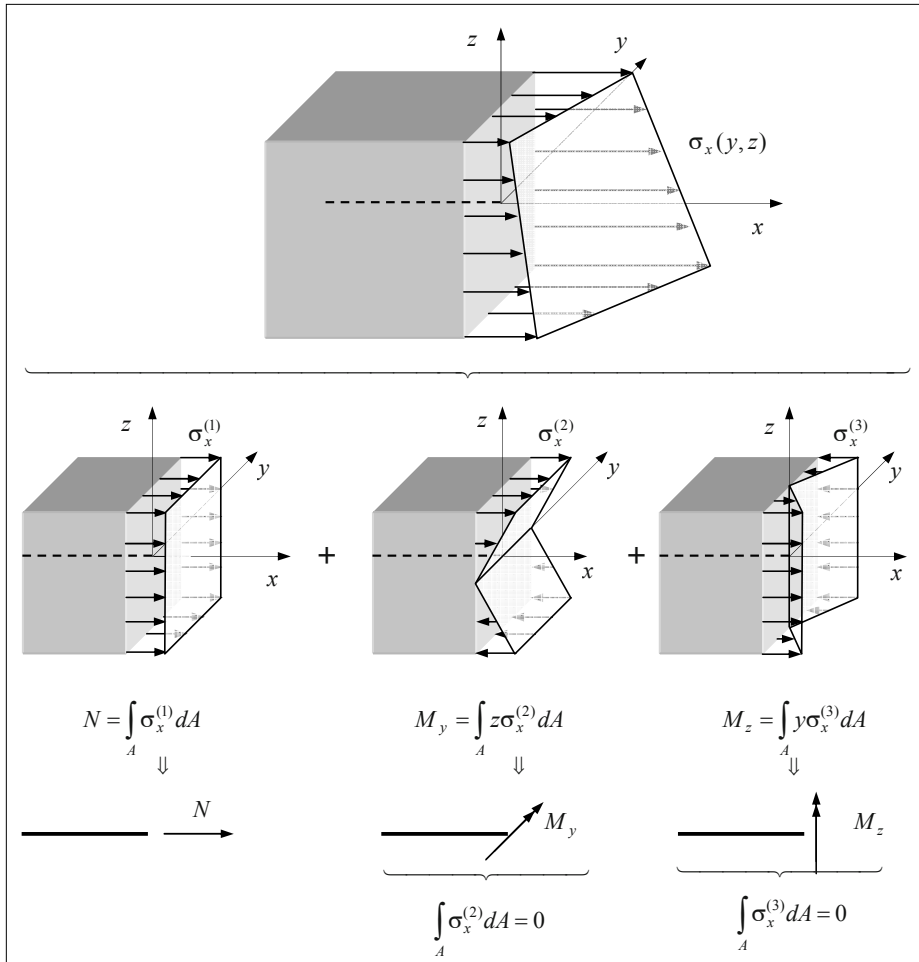
Figure 7.24: The internal normal force and the bending moments.
