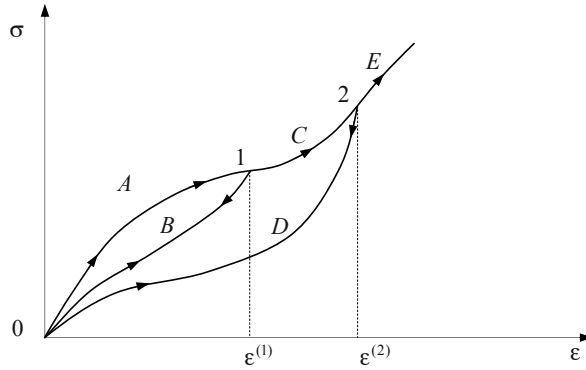
Figure 11.14: Mullins effects.
