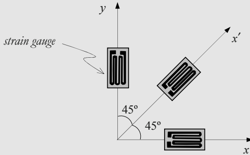
Figure 7.20: Strain rosette.
