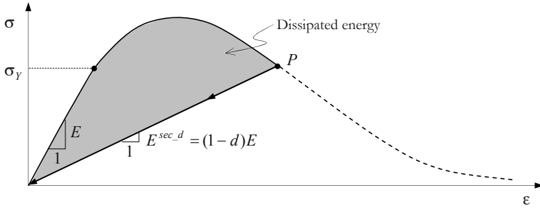
Figure 11.4: Stress-strain curve.
