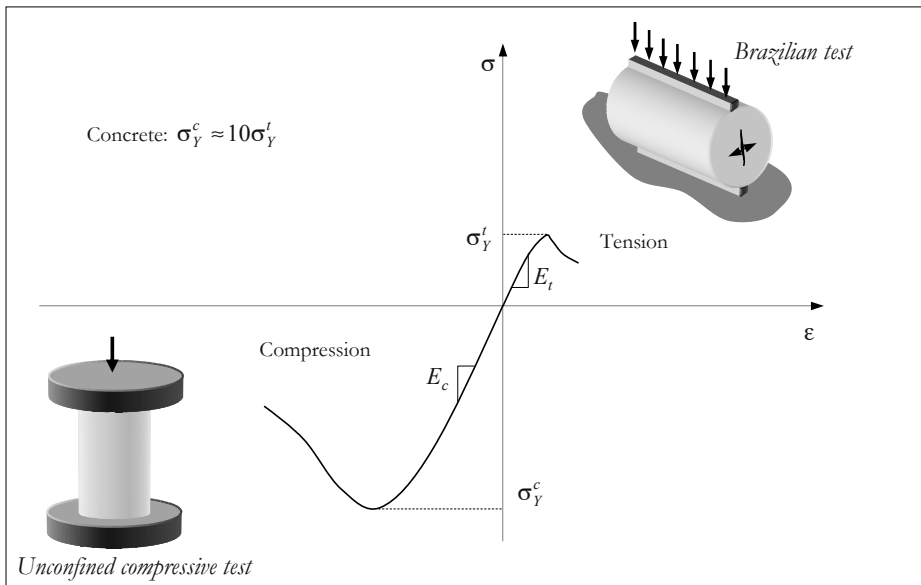
Figure 6.14: The stress-strain curve for concrete.
