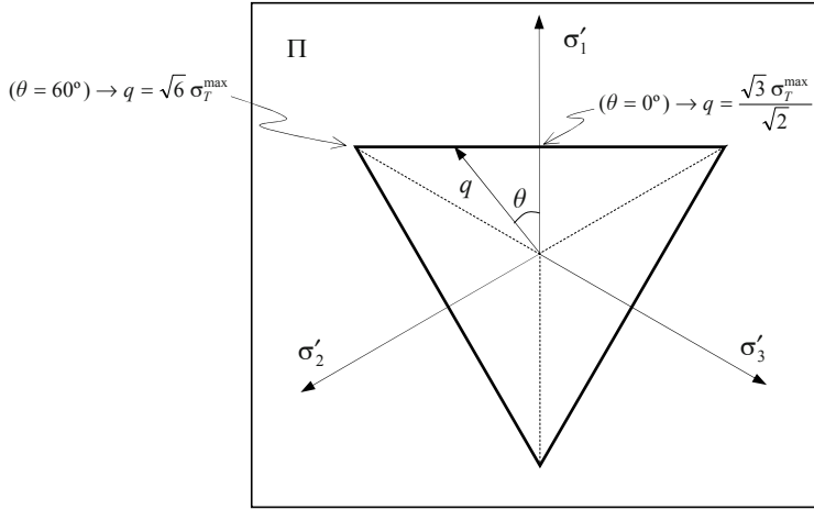
Figure 9.24: The Rankine yield criterion – Nadai's plane.
