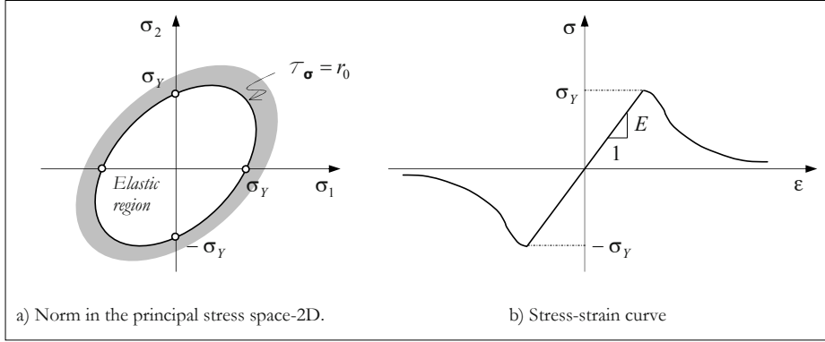
Figure 11.9: Damage surface in 2D and the uniaxial stress-strain curve for model I.
