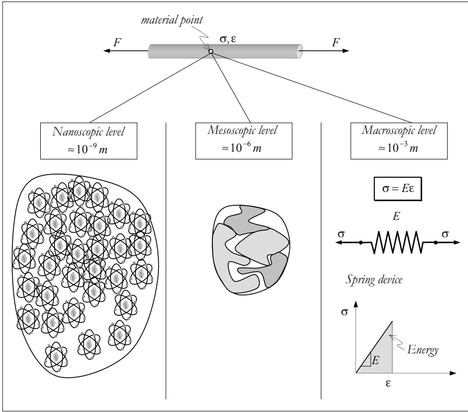
Figure 6.23: Spring device.
