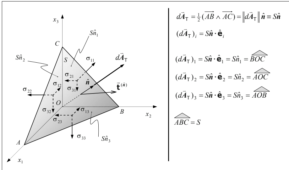
Figure 3.10: The traction vector in an arbitrary plane.
