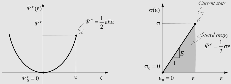
Figure 6.4: Stress-strain relationship (a one-dimensional case).
