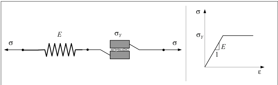
Figure 6.26: The rheological model for perfect elastoplasticity.
