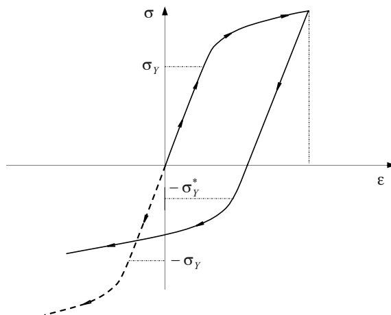
Figure 6.15: The Bauschinger effect.
