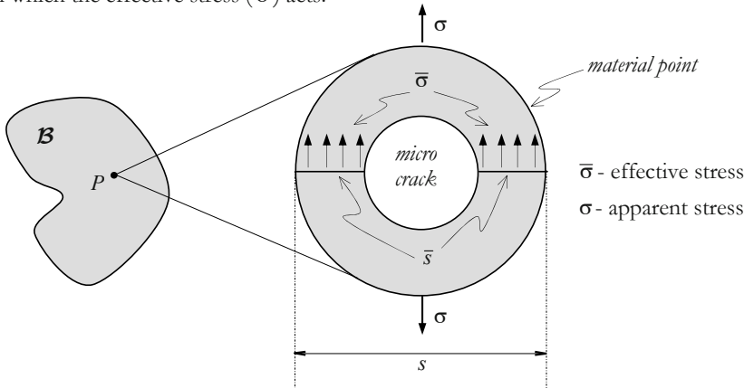
Figure 11.1: Continuum with microcracks.
