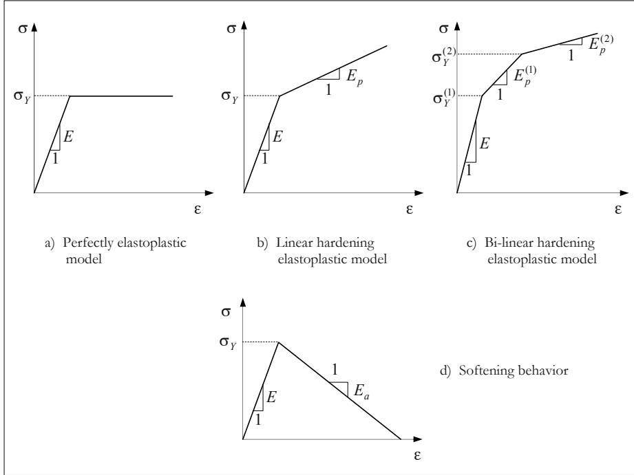
Figure 6.12: Some idealizations of the stress-strain curve.
