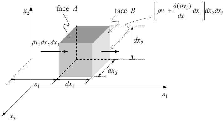
Figure 5.5: Conservation of mass in a differential volume element.
