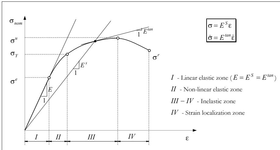
Figure 6.10: Stress-strain curve.
