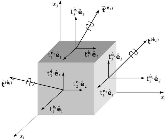
Figure 3.7: Representation of the three tractions in the Cartesian basis.
