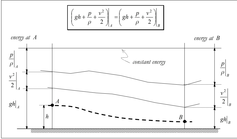
Figure 12.6: Energy vs. the Bernoulli's theorem.
