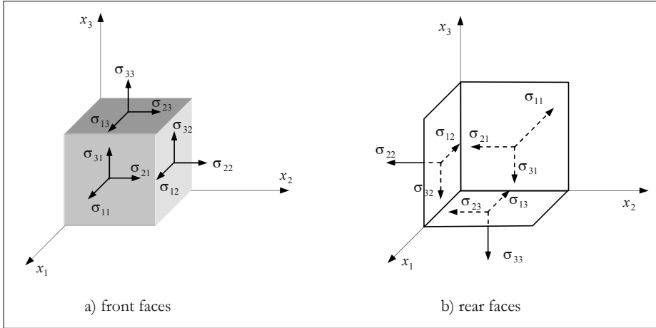
Figure 3.8: Stress state at a point P .
