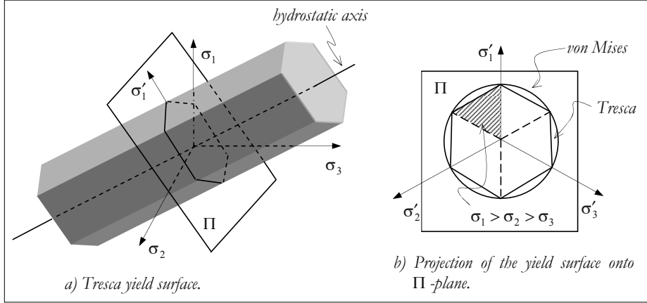
Figure 9.10: Tresca yield surface.
