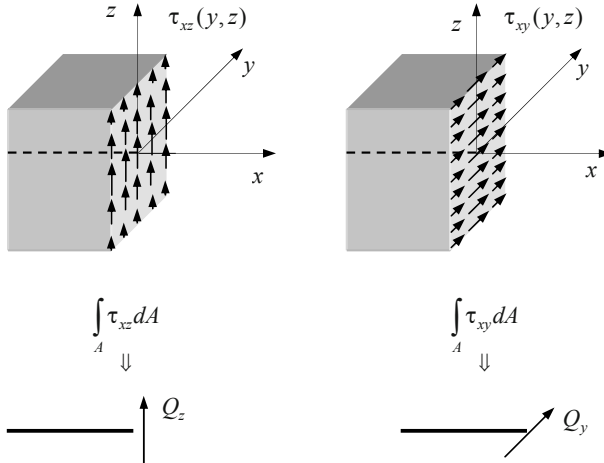
Figure 7.26: The shear stresses – Shear forces.
