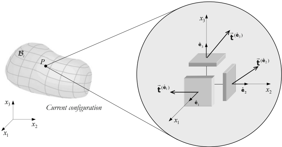
Figure 3.6: The stress state at the point P .
