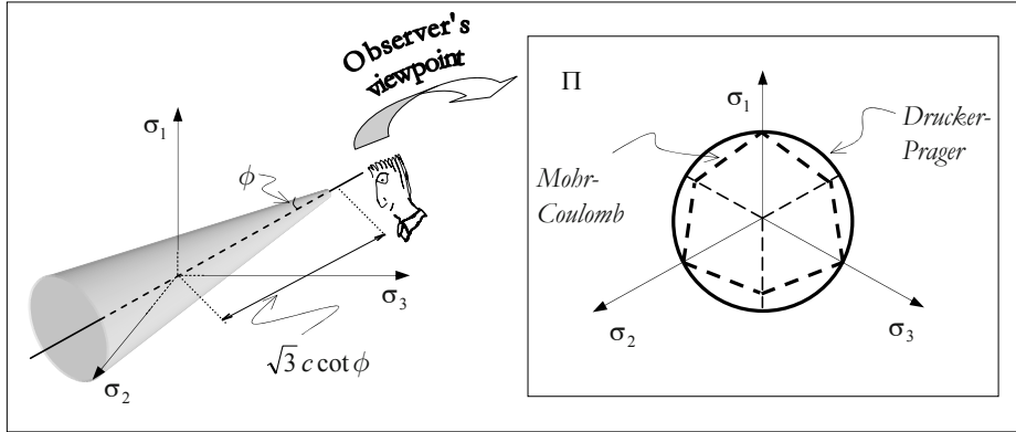
Figure 9.20: Drucker-Prager yield surface.
