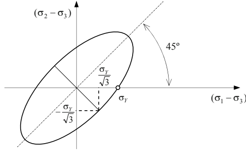
Figure 9.7: The von Mises yield criterion.
