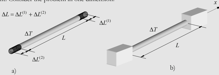
Figure 7.14: Rod under thermal effect.
