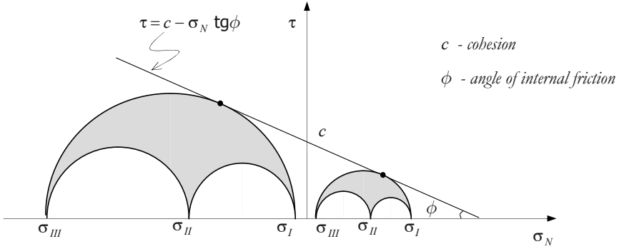
Figure 9.14: Varying the hydrostatic pressure so as to define the Mohr-Coulomb criterion.
