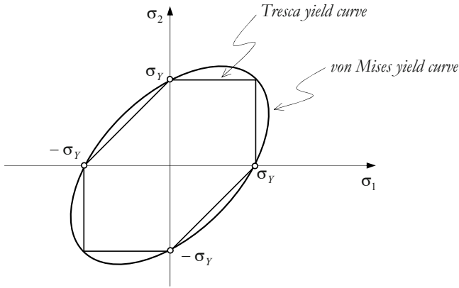
Figure 9.13: The yield curves for von Mises and de Tresca – Plane stress.
