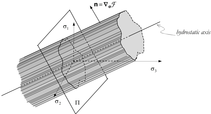
Figure 9.3: Yield surface for isotropic materials independent of pressure.
