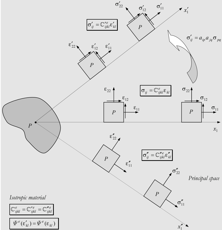
Figure 6.5: Stress-strain relationship (isotropic material).
