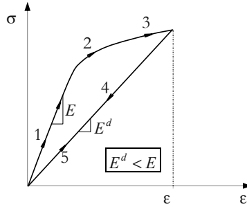
Figure 6.8: Inelastic behavior (damage model).
