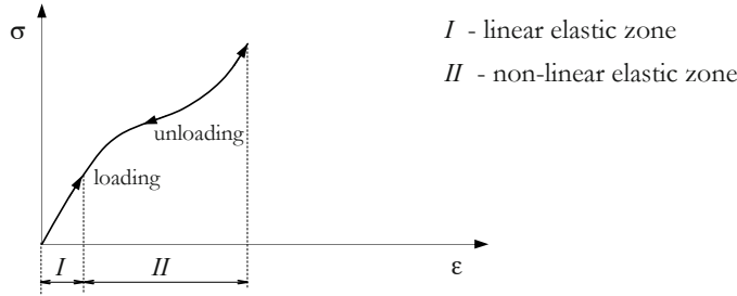
Figure 8.1: The stress-strain curve for elastic materials.
