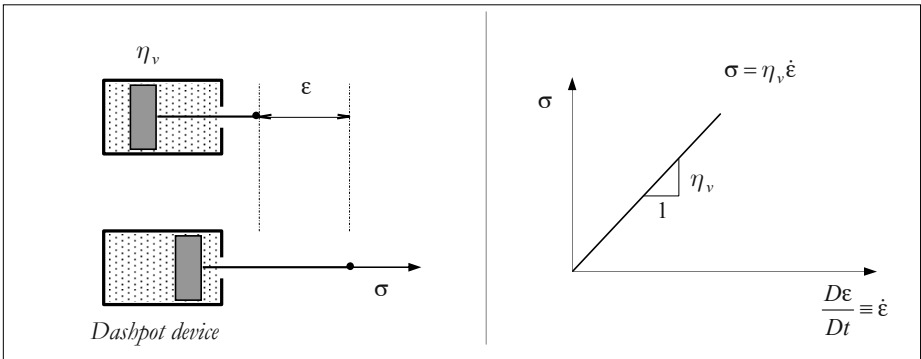
Figure 6.25: Viscous dashpot device.
