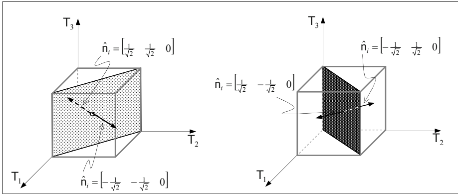
Figure A.5: The maximum relative for T_S , solution (6).
