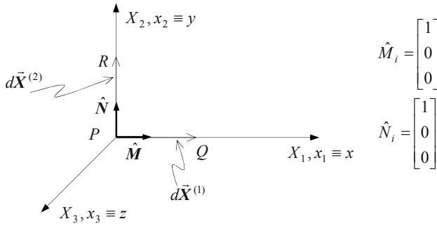
Figure 2.35: Angle change.
