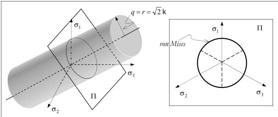
Figure 9.6: Yield surface for von Mises yield criterion (independent of pressure).
