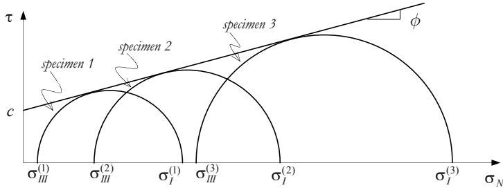
Figure 6.17: Mohr's circle for three specimens – Triaxial test.
