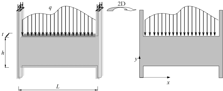
Figure 7.16: Deep beam.
