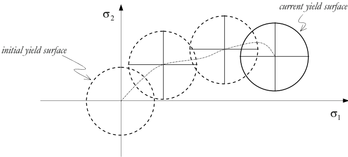
Figure 9.27: Evolution of the yield curve – kinematic hardening behavior.
