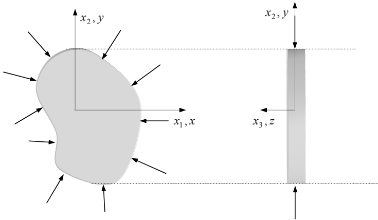
Figure 7.15: Plate
