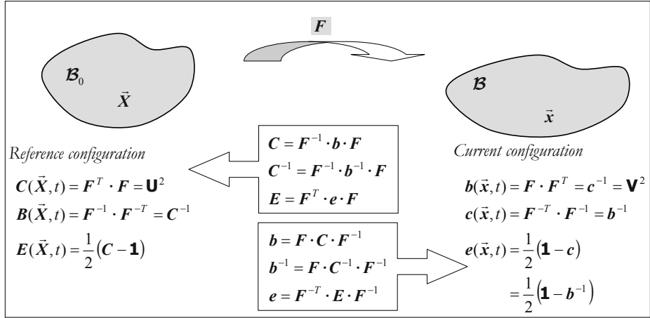
Figure 9.44: Kinematic tensors.
