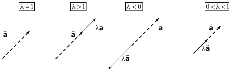
Figure 1.2: Scalar multiplication.
