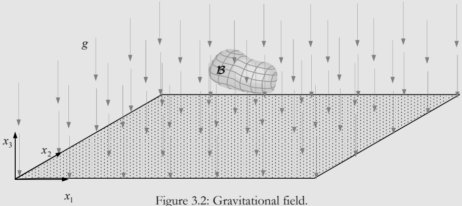
Figure 3.2: Gravitational field.
