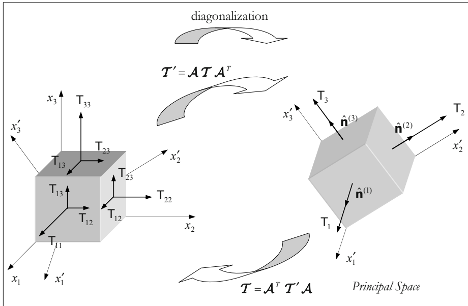
Figure 1.27: Diagonalization.
