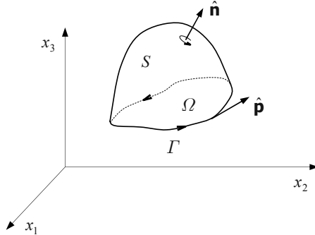
Figure 1.40: Stokes' theorem.
