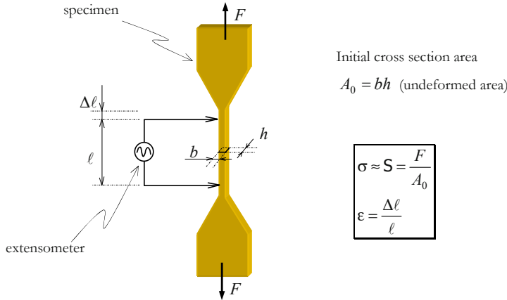
Figure 6.9: A specimen under tensile forces.
