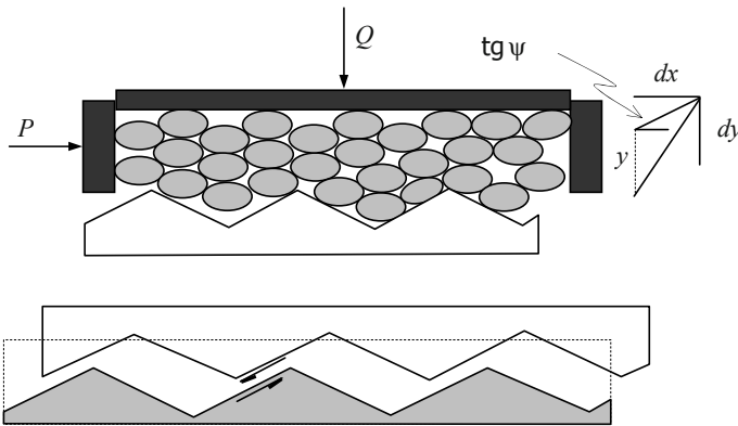
Figure 6.18: Dilatancy.
