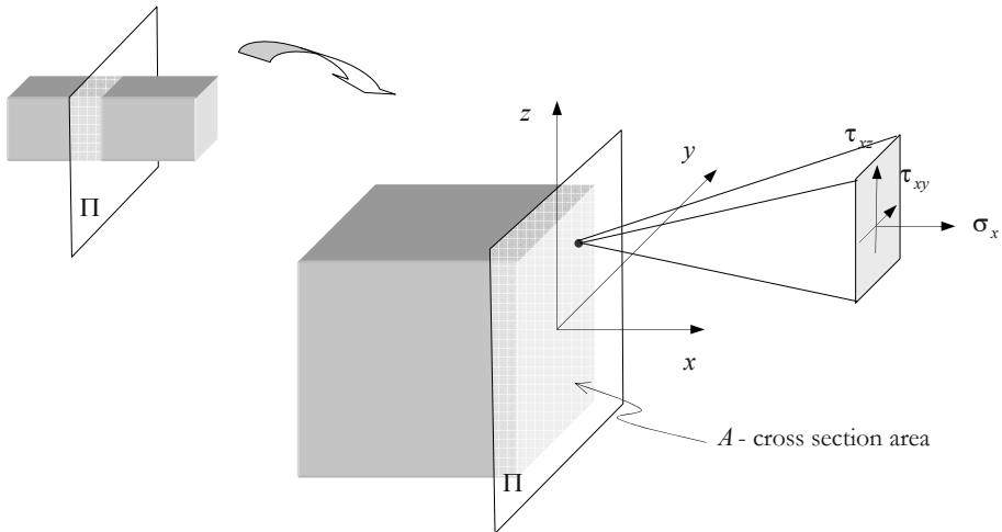
Figure 7.23: Stress at a point in the beam cross section.
