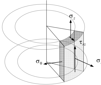
Figure 7.21: Stress components – Axisymmetric solid.
