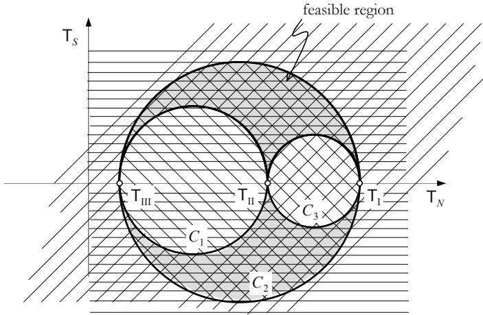
Figure A.10: Mohr's circle – feasible region.
