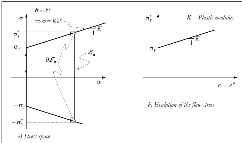
Figure 9.35: Isotropic hardening elastoplastic behavior.
