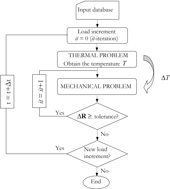
Figure 10.4: Flowchart of the decoupled thermo-mechanical problem.
