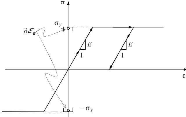
Figure 9.31: Perfect elastoplastic behavior.
