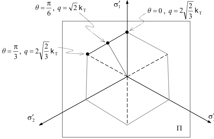
Figure 9.11: Tresca yield surface – Projection of the surface onto the deviatoric plane.
