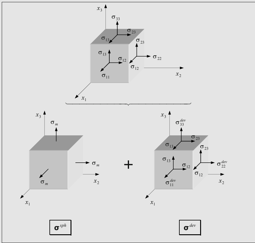
Figure 3.15: The spherical and deviatoric part of \boldsymbol{\sigma} .
