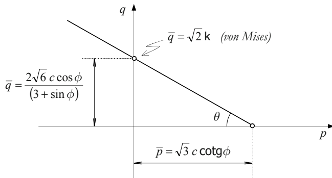
Figure 9.19: Pressure vs. deviatoric part – Drucker-Prager criterion.
