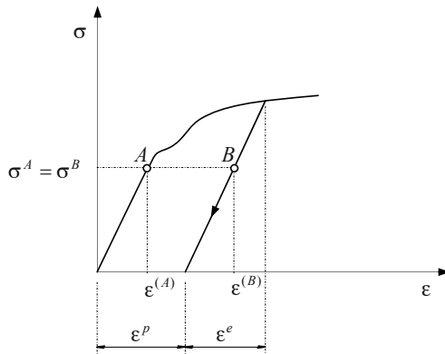
Figure 9.38: Plasticity – dependence of the load history.
