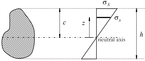
Figure 7.25: Normal stress distribution in the beam cross section.
