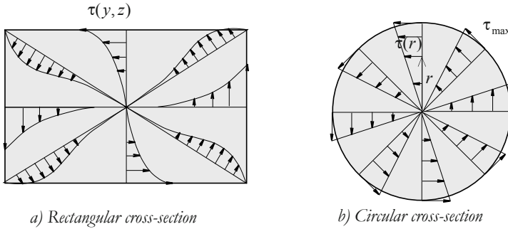
Figure 7.28: Distribution of the shear stress.
