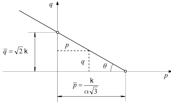
Figure 9.21: Pressure vs. deviatoric part – the Drucker-Prager criterion.
