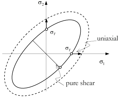
Figure 9.8: The von Mises yield criterion – the state of plane stress.
