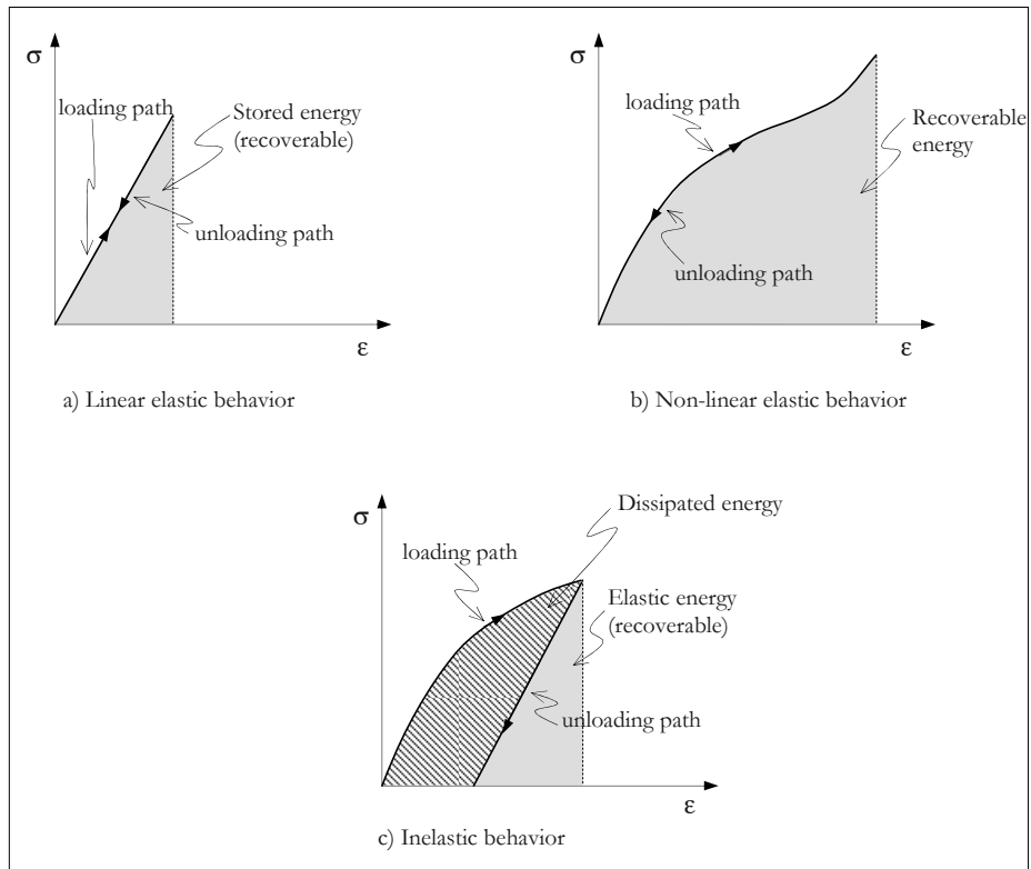
Figure 6.6: Behavior of solids (a one-dimensional case).
