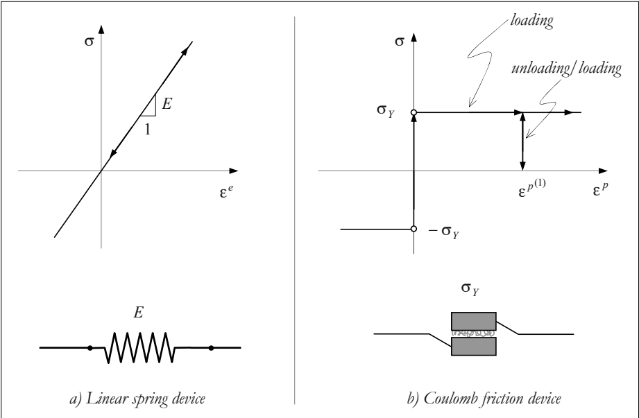
Figure 9.29: Behavior of some devices.
