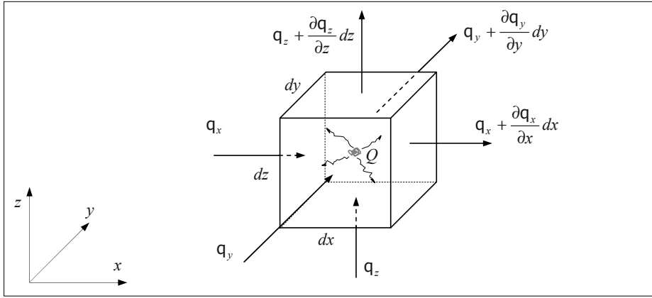
Figure 5.13: Source and heat flux in a differential volume element.
