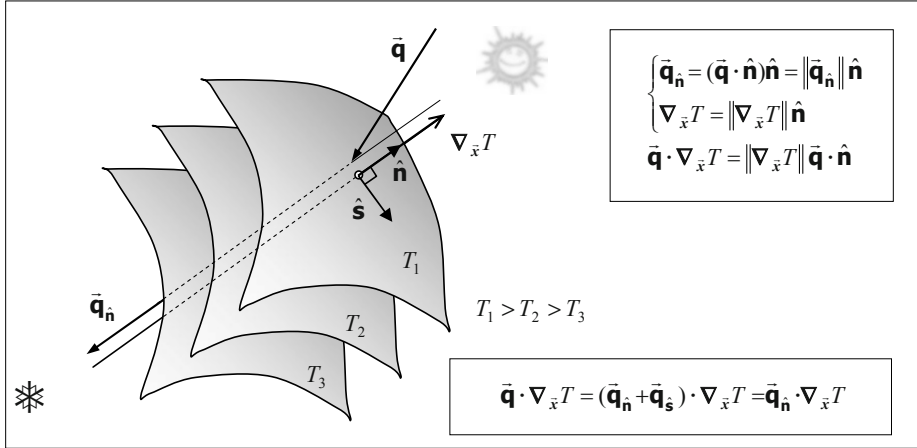
Figure 5.10: Temperature gradient and heat flux vector.
