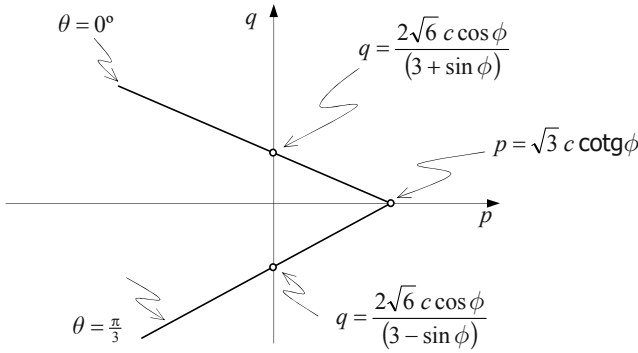
Figure 9.17: Pressure vs. deviatoric part – Mohr-Coulomb yield criterion.
