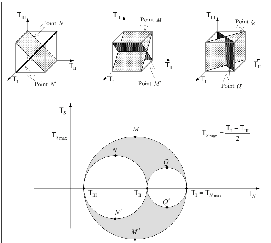
Figure A.11: Mohr's circle.
