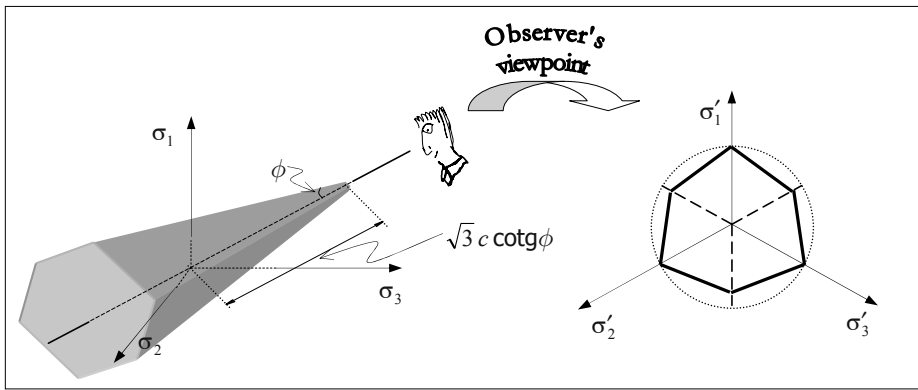
Figure 9.18: The Mohr-Coulomb yield surface.
