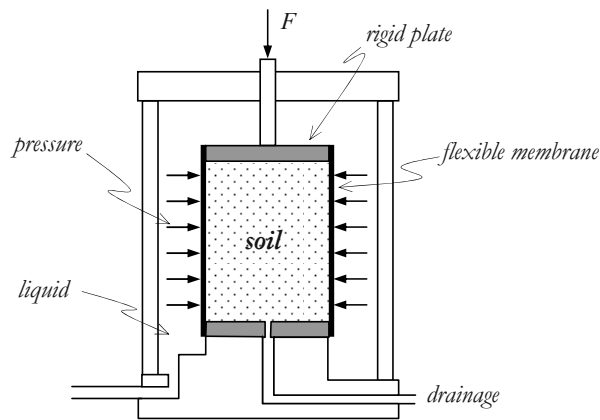
Figure 6.16: Cross section of the triaxial compression test apparatus.
