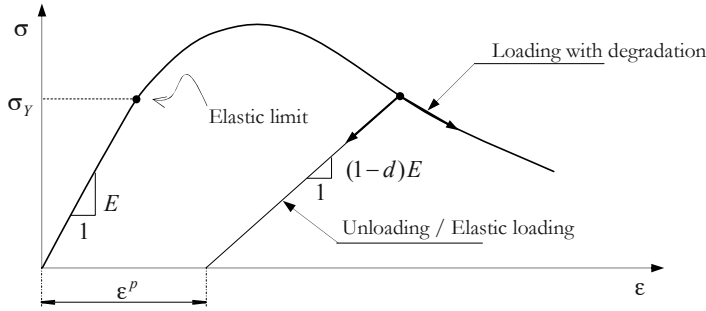
Figure 11.13: Stress-strain curve for elasto-plastic damage model.
