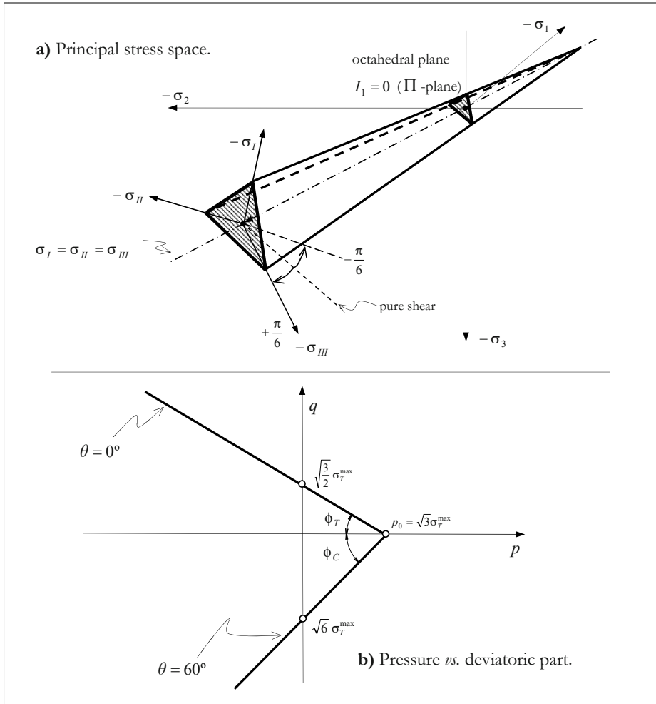
Figure 9.25: The Rankine yield surface.
