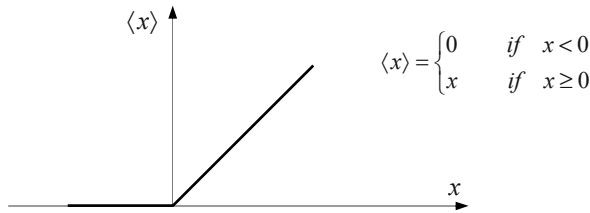
Figure 11.10: Ramp function.
