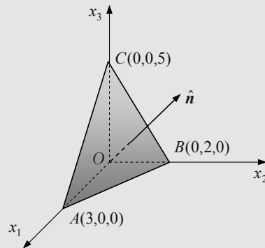
Figure 3.11: Plane ABC .
