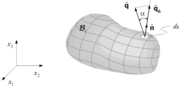
Figure 5.2: Flux vector.
