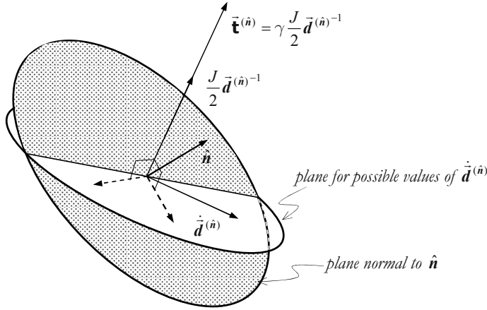
Figure 8.6: Incompressibility restriction.
