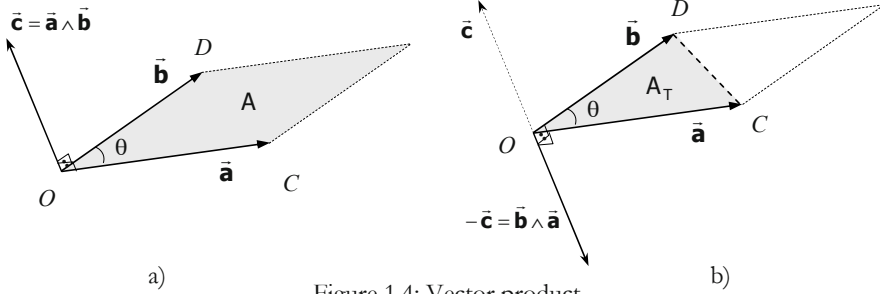
Figure 1.4: Vector product.
