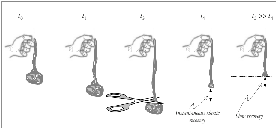
Figure 6.20: Viscoelastic behavior.
