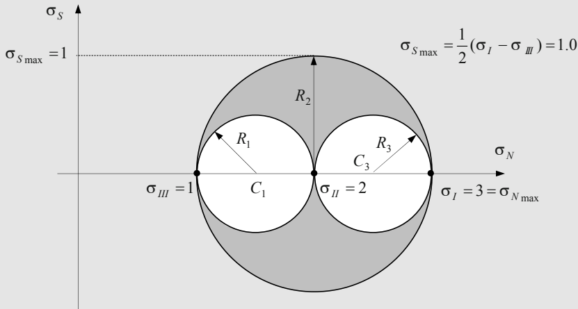
Figure 3.14: Mohr's circle in stress at the point P .
