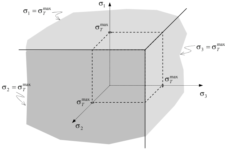
Figure 9.22: The Rankine criterion.
