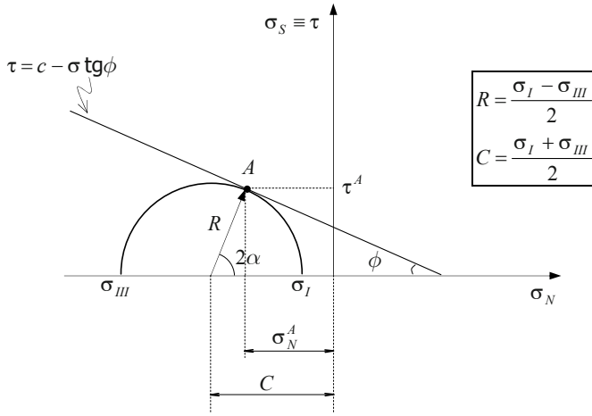
Figure 9.16: Mohr-Coulomb criterion.
