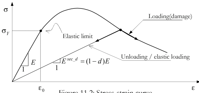
Figure 11.2: Stress-strain curve.
