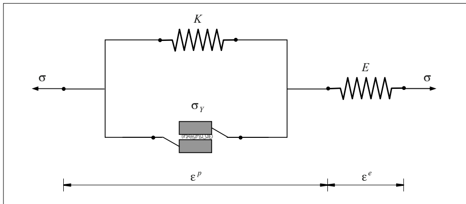
Figure 9.33: The rheological model for the isotropic hardening elastoplastic model.
