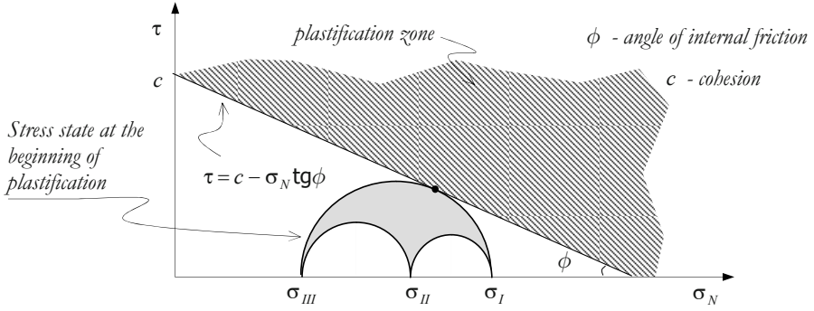
Figure 9.15: Mohr-Coulomb yield criterion.
