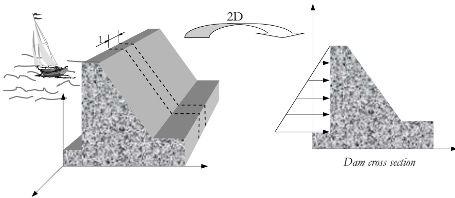
Figure 7.18: Dam.
