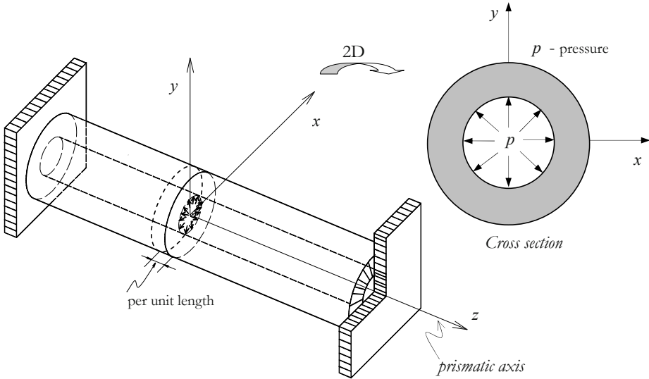
Figure 7.17: Cylinder under pressure.
