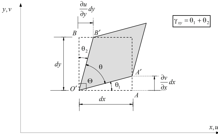
Figure 2.38: Shear strain (small deformation regime).
