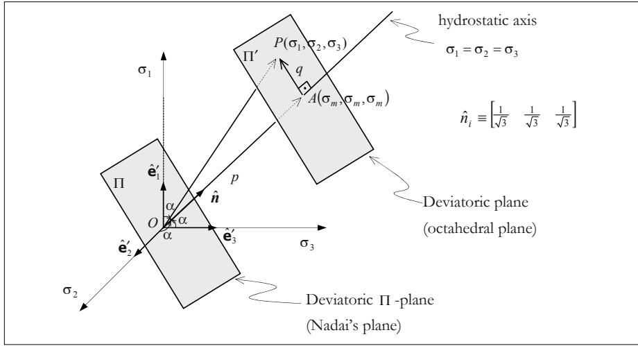
Figure 9.4: Haigh-Westergaard stress space.
