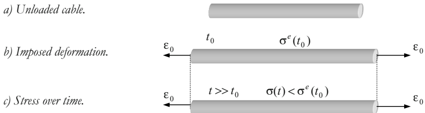
Figure 6.22: Relaxation phenomenon.
